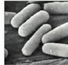
(A) Escherichia coli K-12 4,639,221 nucleotide pairs
